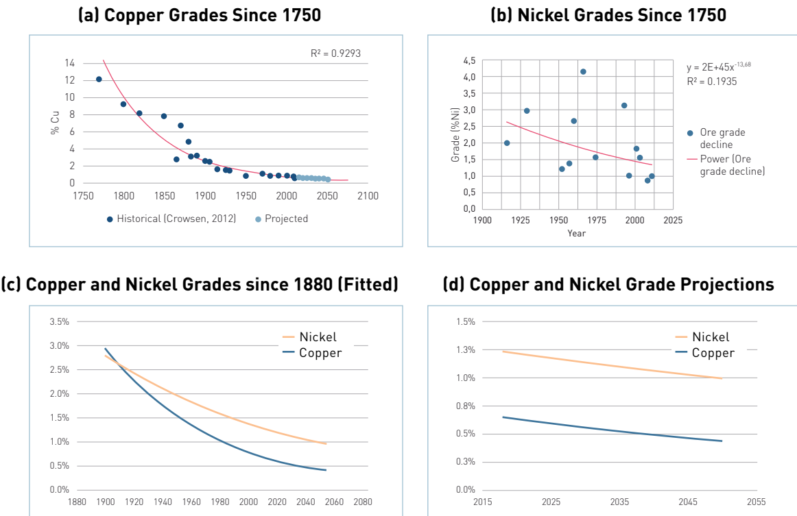
Figure 42. Historical and Fitted Copper and Nickel Ore Grades (Sulfides and Laterites) 160
