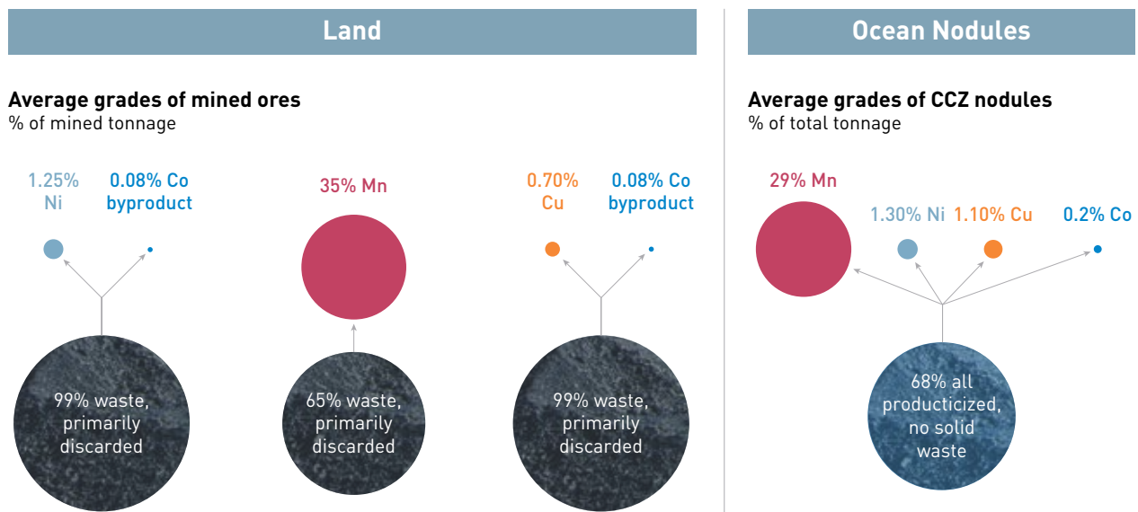
Figure 51. Four Times More Ore Required for Land-Ore Metal Production; Nodules Zero Waste
