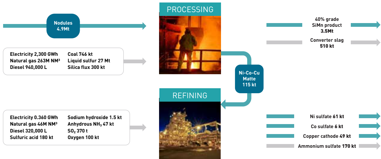
Figure 31. Sample Material Flows for 4.9 Mt/Year Nodule Processing and Refining Plant
